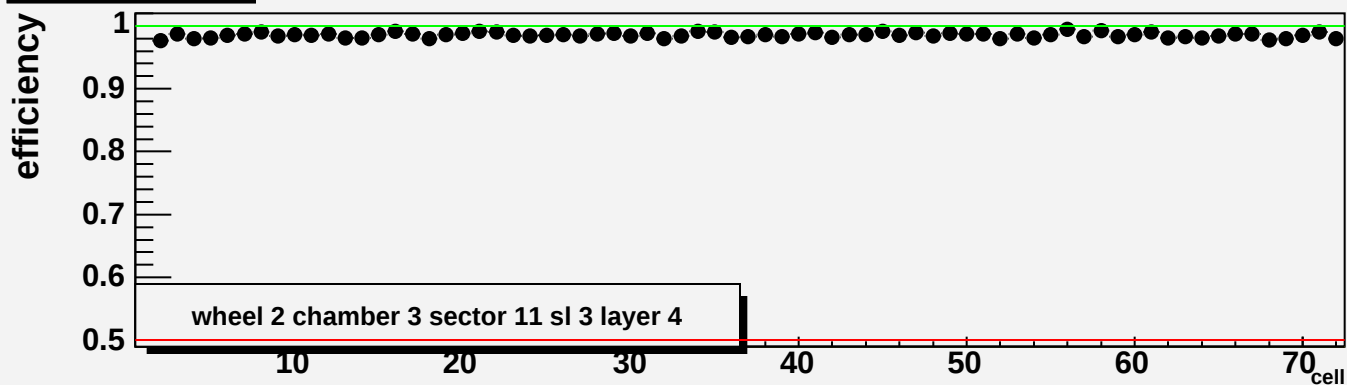
Efficiency in layer 11
