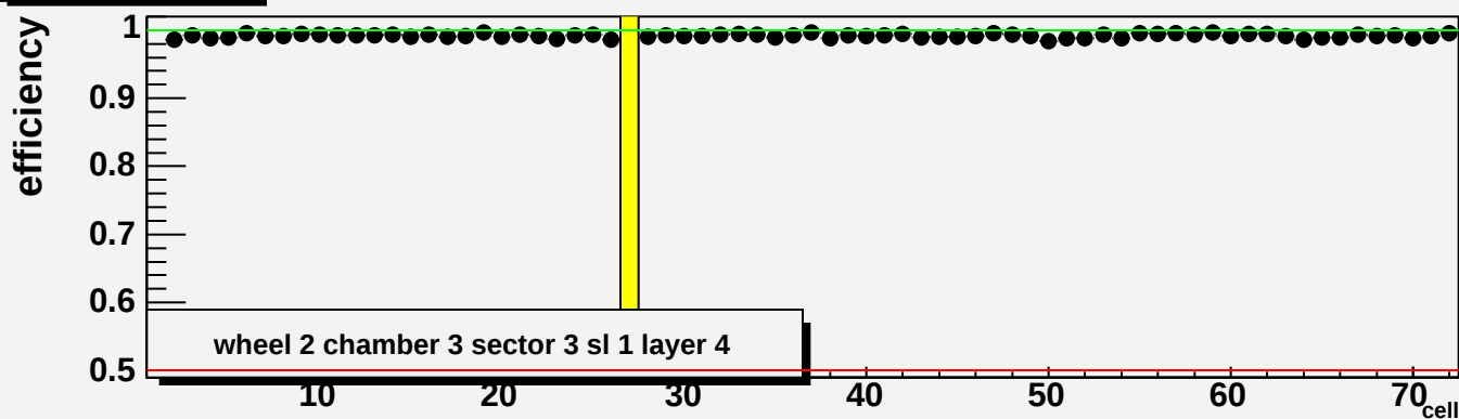
Efficiency_in_layer_3
