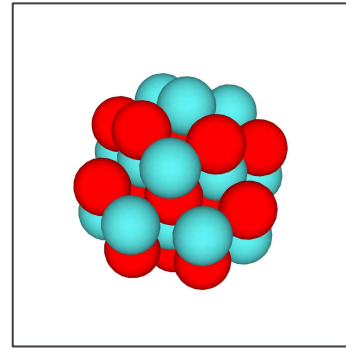
Nucleo atomico ~ 10^{-12} cm
