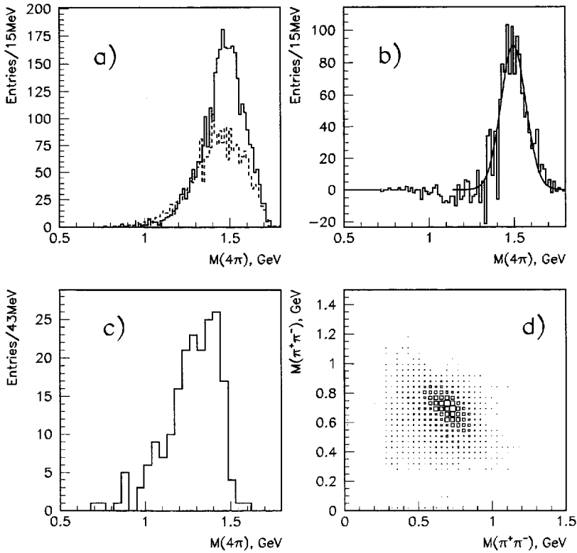
Fig. 14. Invariant masses of the 4\pi system in the reaction \bar{p}d \rightarrow 3\pi^- 2\pi^+ p . (a) The solid line corresponds to the invariant mass of the 2\pi^+ 2\pi^- system and the dashed line is for the \pi^+ 3\pi^- one. (b) Difference spectrum obtained after subtraction of the background 3\pi^- \pi^+ from the 2\pi^+ 2\pi^- distribution. (c) The invariant mass of 4\pi for events with high proton momenta ( P > 400 MeV/c). (d) The scatter plot of the invariant masses of dipions \pi^+ \pi^- (for events with P < 200 MeV/c).
