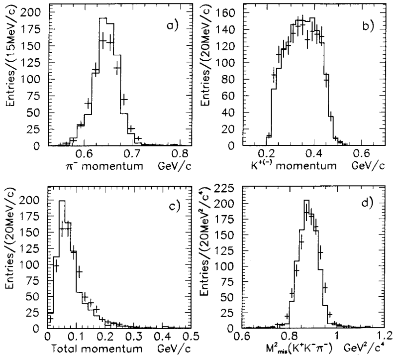
Fig. 5. Comparison between the results of the Monte Carlo simulations (crosses) and the experimental data (solid line). (a) Momentum distribution of negative pions; (b) momentum distribution of kaons; (c) distribution of the total momentum of particles in JDC \vec{P}_{\text{tot}} = \vec{p}_1 + \vec{p}_2 + \vec{p}_3 ; (d) missing-mass-squared distribution.
