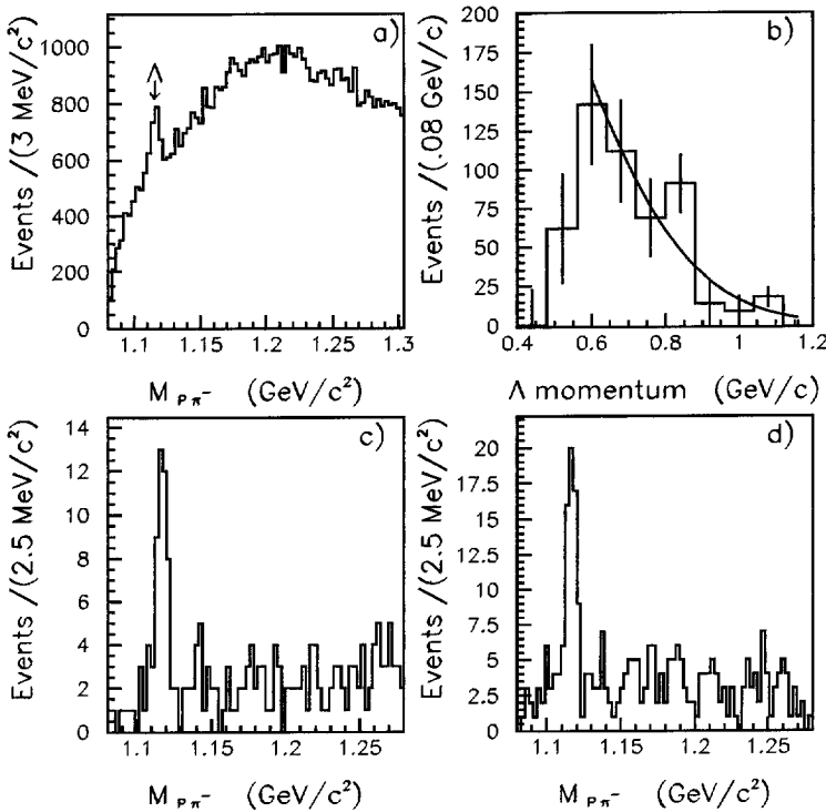
Fig. 17. (a) Invariant mass of p\pi^- pairs. (b) \Lambda -momentum distribution (not corrected for the acceptance). (c) Invariant mass of p\pi^- pairs in the reaction \bar{p}d \rightarrow \Lambda K^+ \pi^- . (d) Invariant mass of p\pi^- pairs in the reaction \bar{p}d \rightarrow \Lambda K^+ \pi^- \pi^0 .
