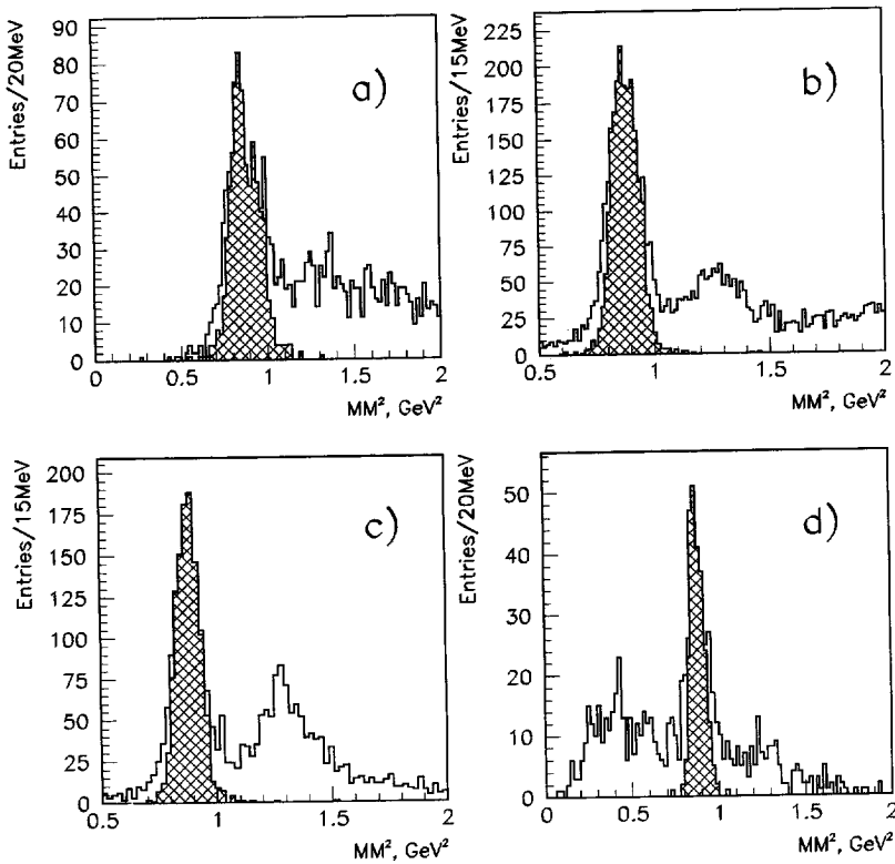
Fig. 10. The distributions of the missing mass squared M_{\text{mis}}^2 for the reactions with (a) 3, (b) 4, (c) 5 and (d) 6 charged pions in the final state. M_{\text{mis}}^2 = (M_p + M_d - \sum_i E_i)^2 - P_{\text{tot}}^2 , where E_i are the energies of charged pions and P_{\text{tot}} is the total momentum of the charged pions. The solid lines correspond to the distributions when the nucleon-spectator cut of P_{\text{tot}} < 200 MeV/c was applied. The hatched histograms correspond to the events which have the confidence level for the investigated hypothesis greater than 10%.
