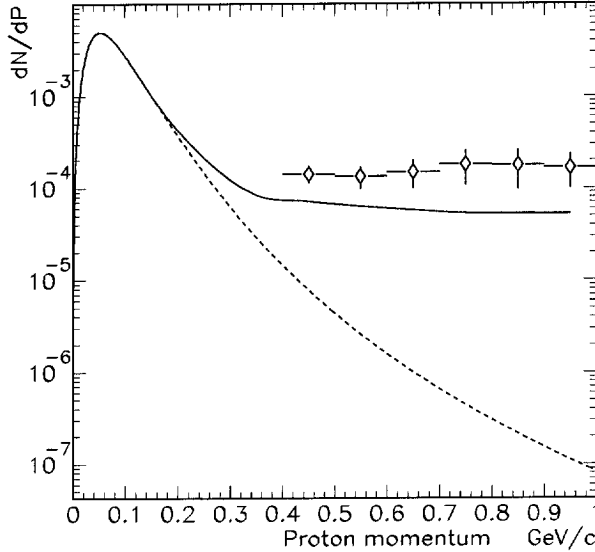
Fig. 8. The yield of \omega for different proton momenta. The solid line corresponds to the result of the calculations of Lev and Buzatu [27] normalized to the experimental yield of \omega\pi in the proton-spectator region. The dashed line corresponds to the calculations where rescattering of annihilation mesons was not taken into account.
