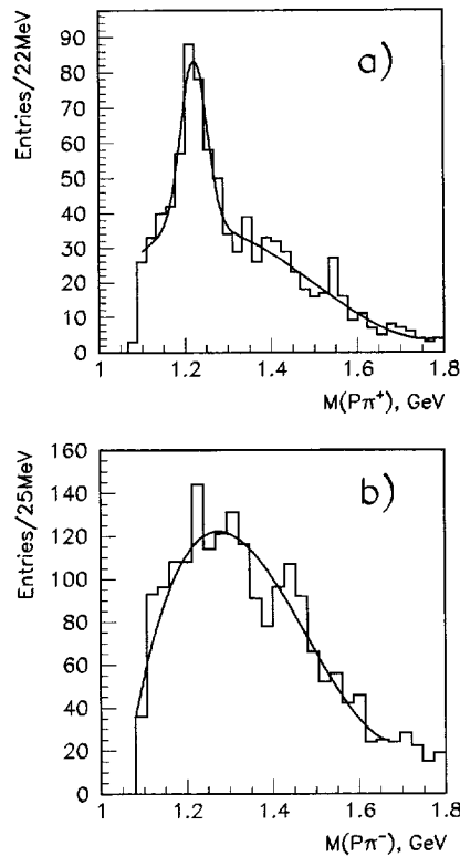
Fig. 16. The invariant-mass distributions of (a) the \pi^+p and (b) the \pi^-p system in the reaction \bar{p} + d \rightarrow \pi^+ + 2\pi^- + p + x\pi^0 , x = 0, 1, 2, \dots , for protons with momenta P > 400 MeV/ c .
