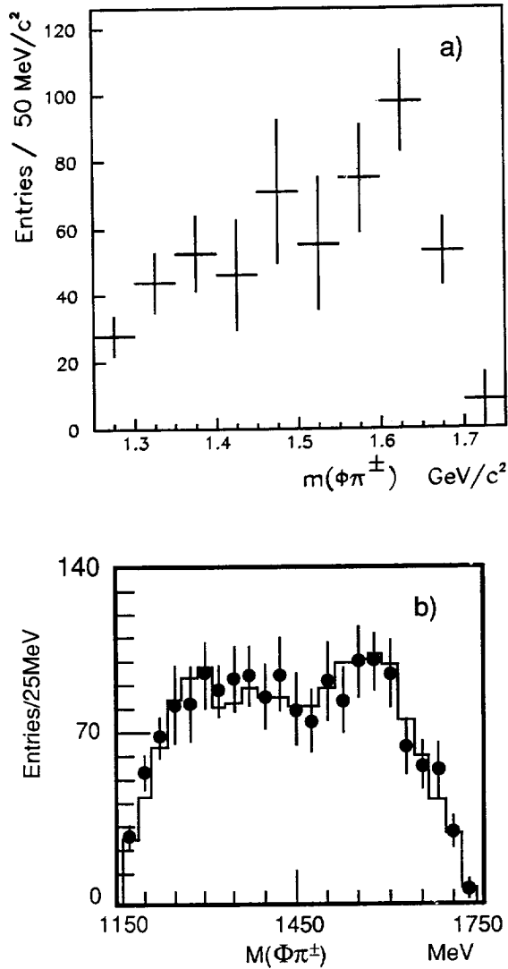
Fig. 9. The invariant-mass distribution of the \phi\pi^\pm system in p\bar{p} annihilations at rest in gaseous hydrogen. The data in (a) are from the OBELIX and (b) from the ASTERIX Collaborations.
