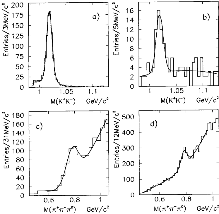
Fig. 3. Invariant-mass distribution of the K^+K^- system in the reaction \bar{p} + d \rightarrow \pi^- + K^+ + K^- + p for (a) the proton-spectator region ( P < 200 MeV/c) and (b) for proton momenta P > 400 MeV/c. Invariant-mass distribution of the \pi^+\pi^-\pi^0 system for the reaction \bar{p} + d \rightarrow 2\pi^- + \pi^+ + \pi^0 + p for (c) the proton-spectator region and (d) for high proton momenta.
