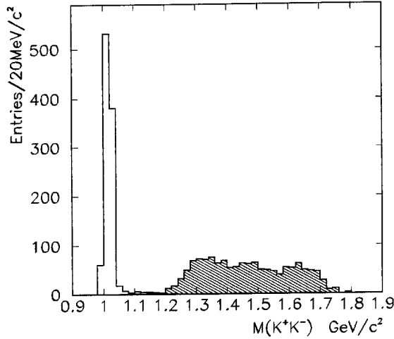
Fig. 4. The invariant-mass distributions of different pairs of particles that passed all selection criteria. The open histogram corresponds to the sum of all three possible combinations of two kaons (13), (23) and (12), the hatched part of the histogram corresponds to the “wrong” combinations (13) and (12).
