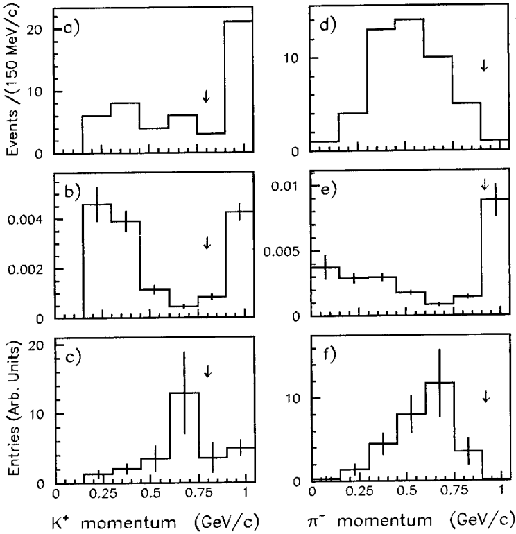
Fig. 18. (a), (d) Distributions of K^+ - and \pi^- -momenta, respectively, for the events under the peak of \Lambda in reaction (40). (b), (e) Distributions of the acceptances for K^+ - and \pi^- -detection. (c), (f) Distributions of K^+ - and \pi^- -momenta, corrected for the acceptances.
