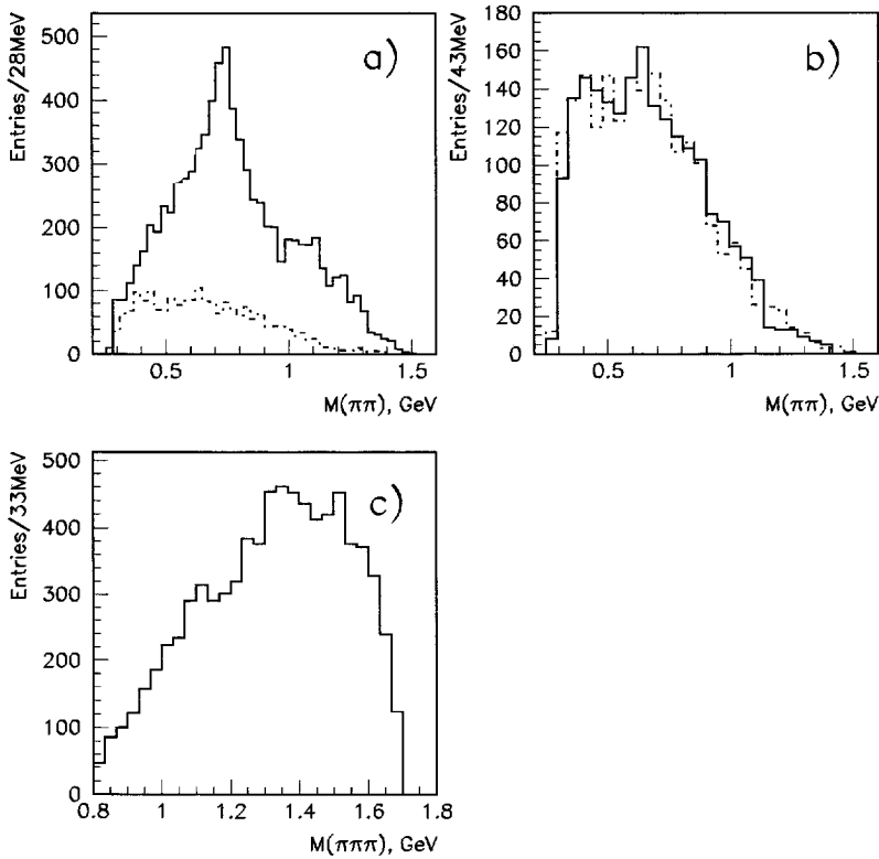
Fig. 13. Invariant-mass distributions of different pion systems in the reaction \bar{p}d \rightarrow 2\pi^- 2\pi^+ n : (a) \pi^+\pi^- (solid line) and \pi^-\pi^- (dashed line); (b) \pi^-\pi^- (solid line) and \pi^+\pi^+ (dashed line); (c) \pi^+\pi^-\pi^+\pi^- .
