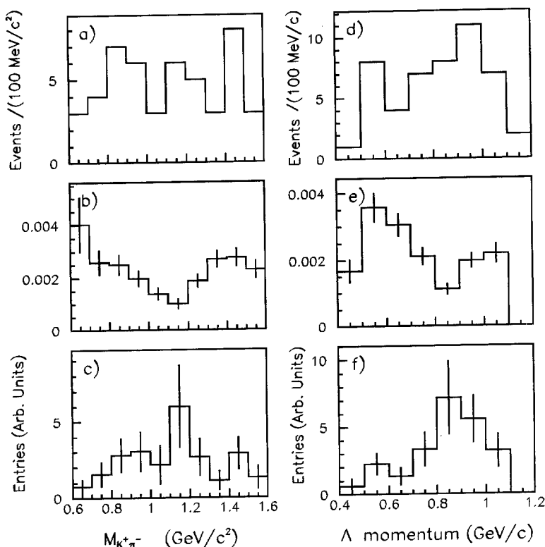
Fig. 19. (a) Distribution of the invariant mass of the K^+\pi^- system for the detected events under the peak of \Lambda in reaction (40). (b) Distribution of the acceptance of the K^+\pi^- system in reaction (40). (c) The reconstructed distribution of the invariant mass of the K^+\pi^- system. (d) The total momentum distribution of p\pi^- pairs for the detected events in reaction (40). (e) Distribution of the acceptance of p\pi^- pairs in reaction (40). (f) The reconstructed distribution of the total momentum of p\pi^- pairs.
