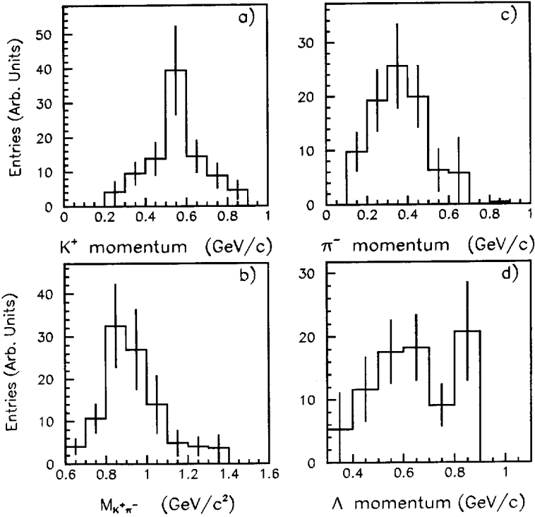
Fig. 20. (a), (c), (d) Distributions of K^+ , \pi^- and \Lambda -momenta in reaction (41), respectively. (b) Distribution of the invariant mass of the K^+\pi^- system in reaction (41).
