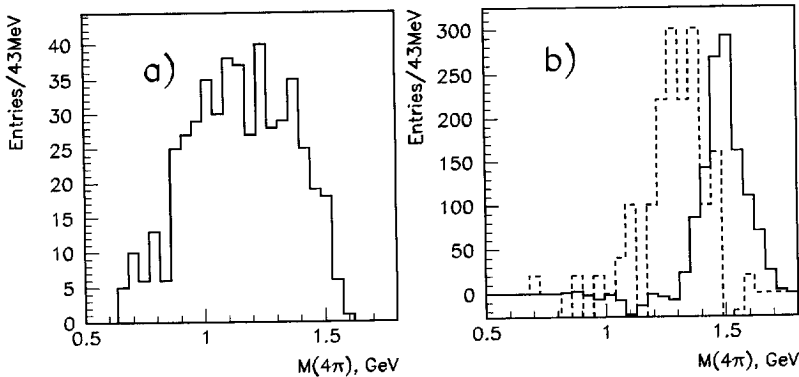
Fig. 15. (a) The Monte Carlo simulation of the invariant-mass distribution of the 4\pi system in the reaction \bar{p}d \rightarrow \pi^- X(1480)p assuming a flat proton-momentum spectrum for P > 400 MeV/c. (b) Difference spectrum of the 4\pi system for the sample with P_{\text{tot}} < 200 MeV/c (solid line) and for the data with P_{\text{tot}} > 400 MeV/c (dashed line). The latter histogram is multiplied by 20.
