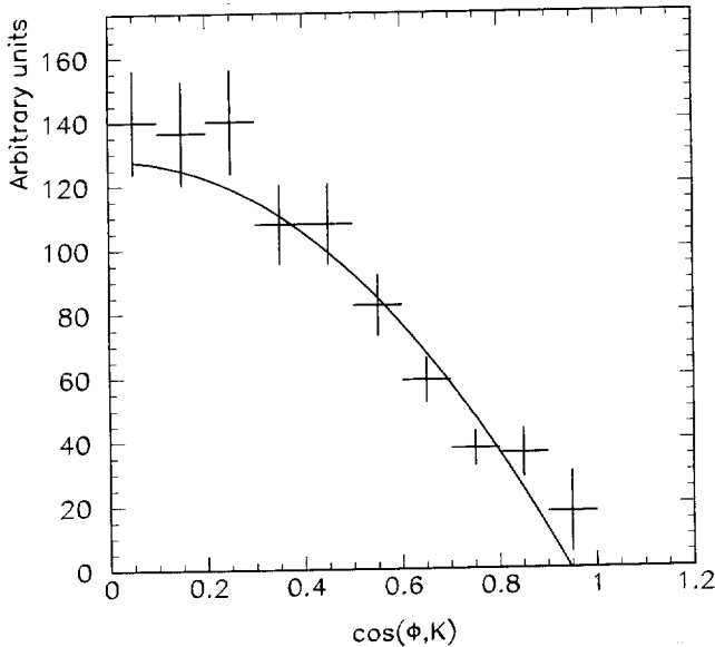
Fig. 6. The \phi \rightarrow K^+ K^- decay angular distribution in the reaction \bar{p} + d \rightarrow \pi^- + \phi + p_s . \theta is the angle between the fast kaon with respect to the \phi -momentum in the K^+ K^- rest frame. The solid line corresponds to the \sin^2 \theta dependence expected for annihilation from the ^3S_1 state.
