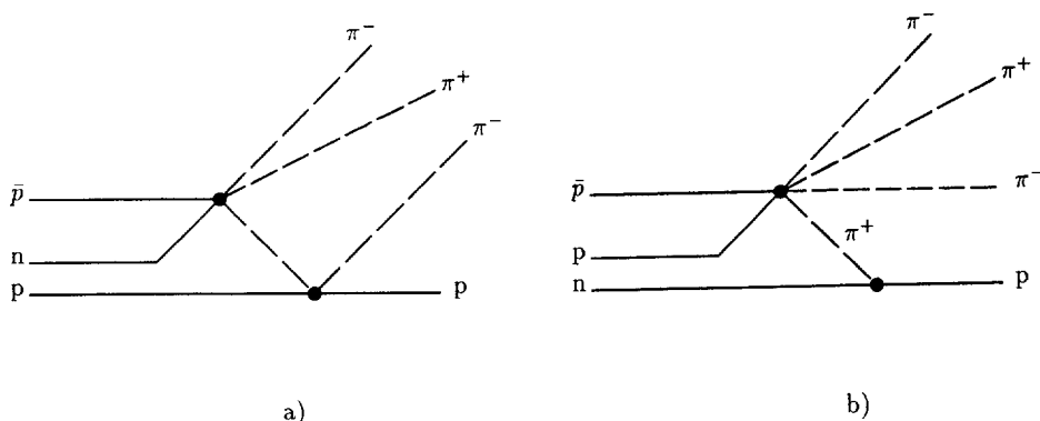
Fig. 12. Diagrams of (a) meson rescattering and (b) the Pontecorvo reaction for the reaction \bar{p}d \rightarrow 2\pi^- \pi^+ p .
