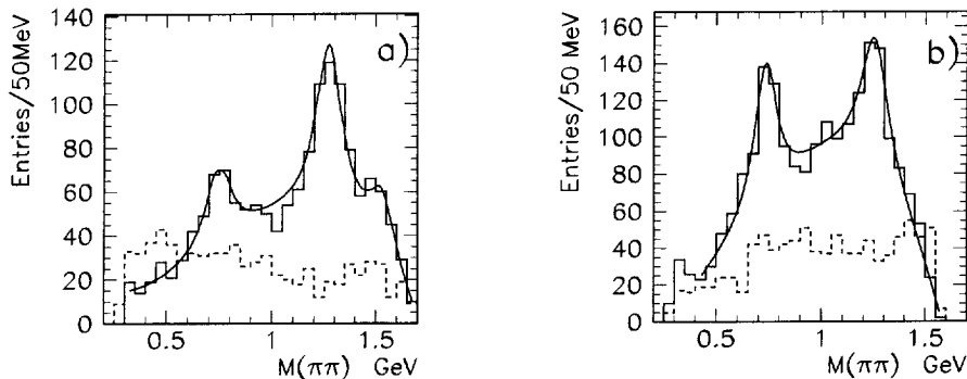
Fig. 11. The invariant-mass distribution of the \pi^+\pi^- (solid line) and \pi^-\pi^- (dashed line) systems in the reaction \bar{p}d \rightarrow 2\pi^-\pi^+p for (a) the proton-spectators ( P < 200 MeV/c) and (b) for annihilation with high-momenta protons ( P > 400 MeV/c).
