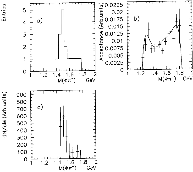
Fig. 7. The invariant-mass distribution of the \phi\pi^- system at high proton momenta ( P > 400 MeV/c). (a) experimental distribution not corrected for the acceptance; (b) acceptance of the apparatus simulated by the Monte Carlo; (c) experimental distribution corrected for the acceptance.
