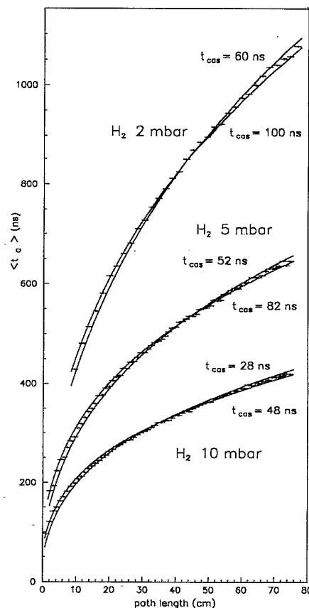
FIG. 3. Mean annihilation time \langle t_a \rangle versus corrected path length with the two limiting behaviors [yielding the dashed lines in Fig. 2(a)], for H_2 at three pressure values.
