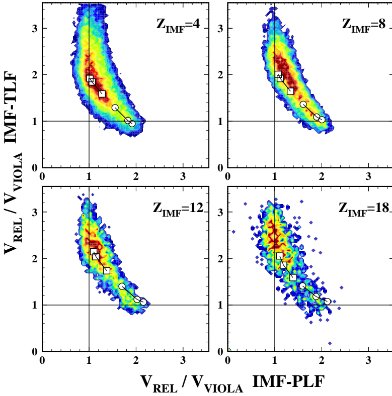
Fig. 1. Correlation between relative velocities V_{rel}/V_{Viola}(IMF, PLF) and V_{rel}/V_{Viola}(IMF, TLF) for different intermediate mass fragments of Z_{IMF} = 4, 8, 12 and 18 . The relative velocities are expressed in units corresponding to the kinetic energy of the Coulomb repulsion of a given binary sub-system. The experimental distributions are compared with simple model calculations assuming that the IMF is released as a result of a two-step neck rupture process taking place 40, 80 or 120 fm/c after reseparation of the primary binary system. Two branches of the calculated correlation system correspond to either projectile breakup (squares) or target breakup (circles); the shortest indicated times \Delta t = 40 fm/c correspond to the location near the diagonal.
