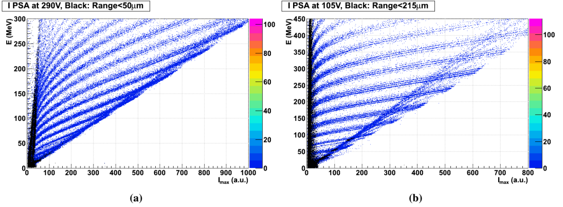
Figure 1: PSA identification plot of E vs. IMAX for a 500\ \mu\text{m} FAZIA silicon operated at different voltages. Left: full depletion voltage, 290 V. Ions are separated in charge but not in mass. Black points are events of ions with a range less than 50\ \mu\text{m} . Right: strong underdepletion voltage, 105 V. Ions are separated in charge and in mass up to Z \sim 10 . Black dots correspond to ions with range less than an arbitrary value of 215\ \mu\text{m} . Some punching through events appear here, more clearly than at 290 V. They survive the CsI(Tl) veto due to a imperfect geometrical match with the silicon pair.
