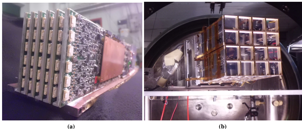
Figure 2: Left: Front view of six FEE cards mounted on the cooling copper plate. The 48 female connectors will receive the corresponding kapton strips from the detectors. Right: Picture of the first FAZIA block mounted for test purposes in the Ciclope scattering chamber at LNS, Catania.
